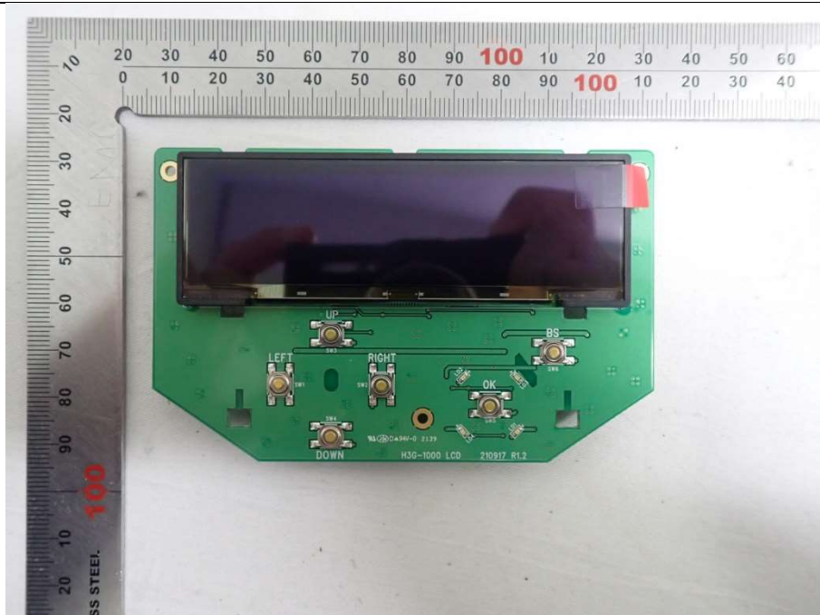
LCD Board (Front)
