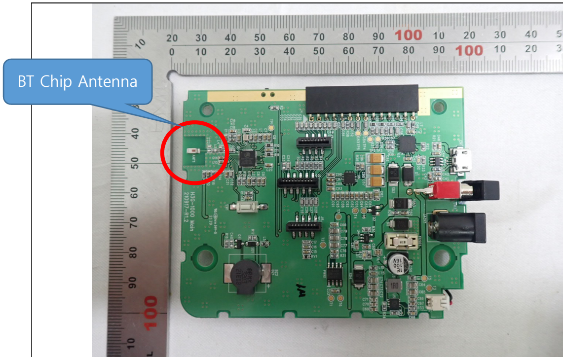
Main Board (Front)
