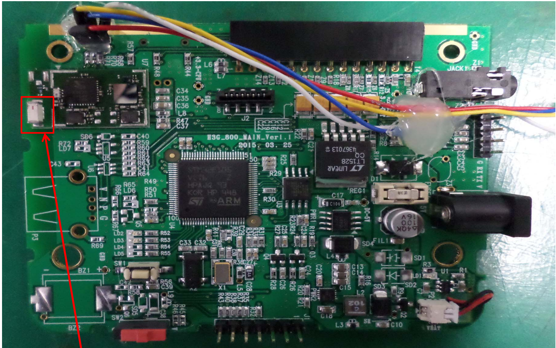
BT Antenna
