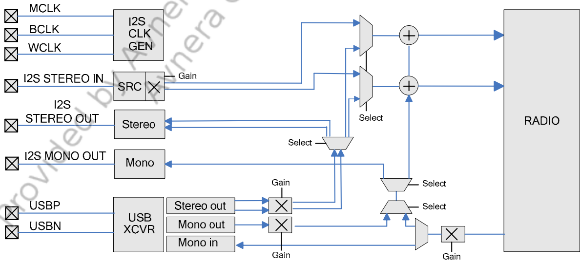
Figure 1-3 AV6301 Audio Routing
