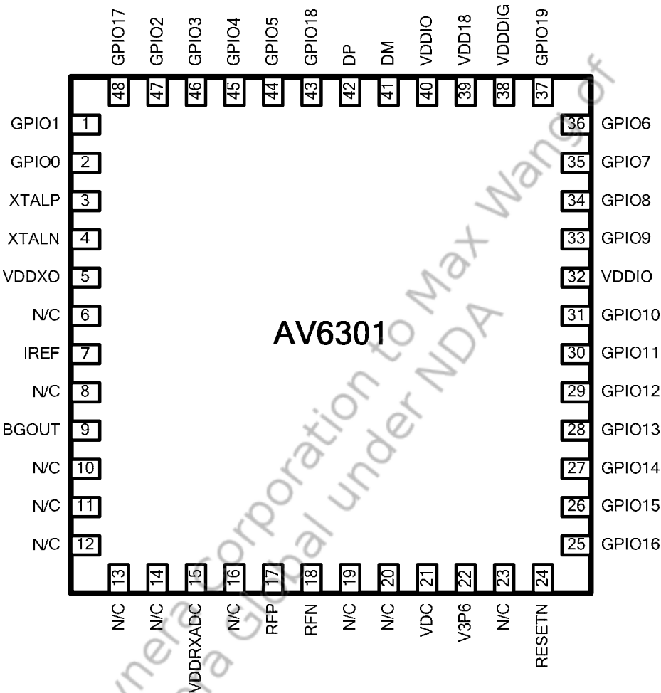
Figure 2-1 AV6301 Pin Diagram
