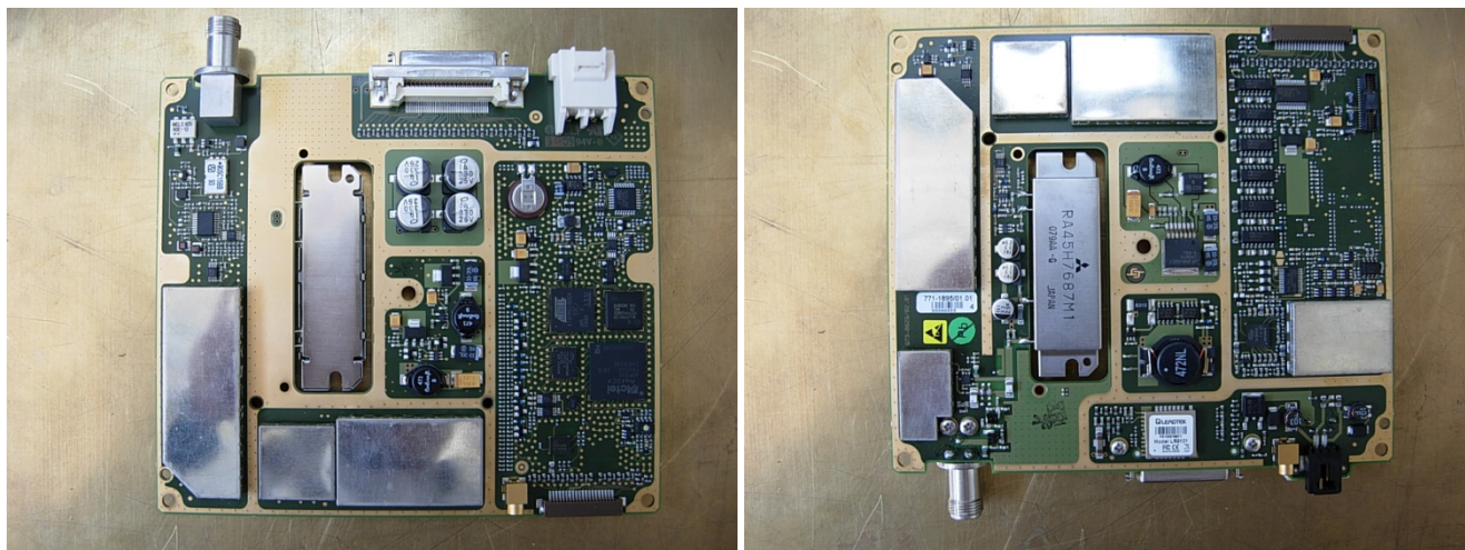
Figure 7: Boards Pictures
