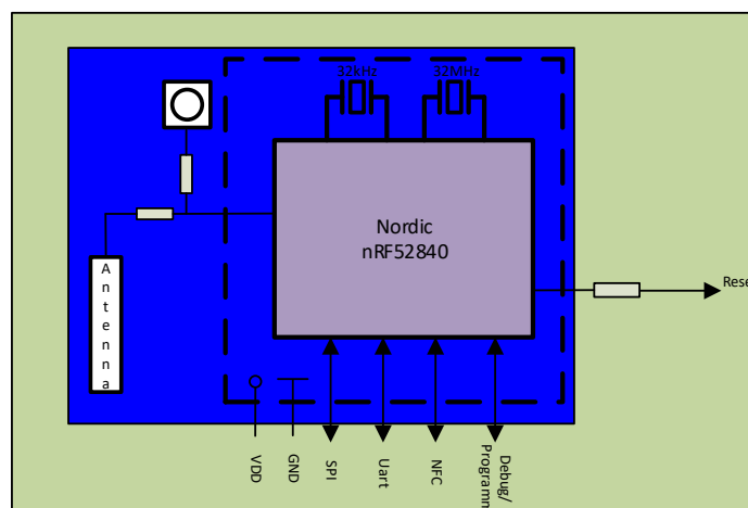
Figure 1.2-2:Block Diagram Dräger BT Modul 17x10mm
