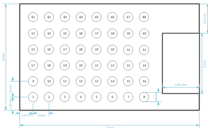
Figure 3.2-1: BT02 Module Pinout (Top View)
