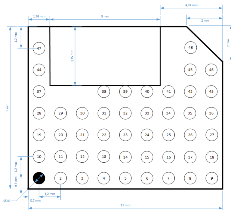
Figure 3.1-1: BT01 Module Pinout (Top View)
