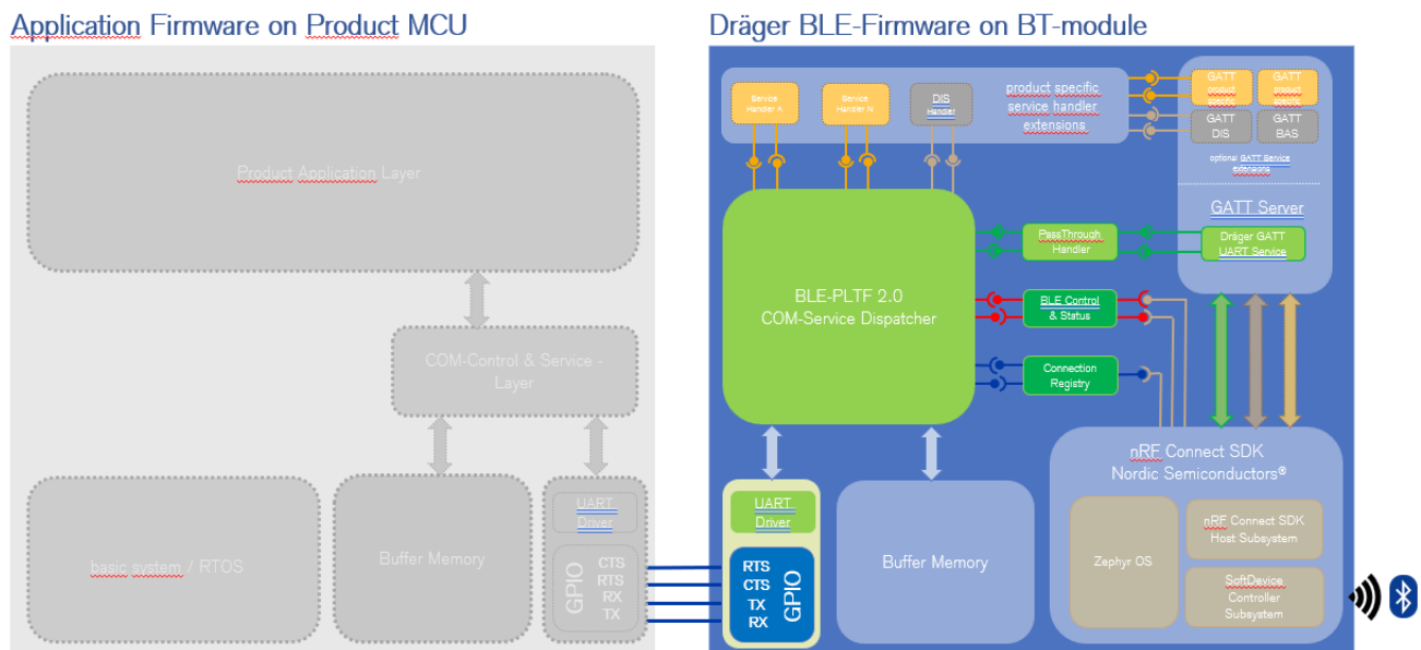
Figure 1.3-1: software architecture with decomposition of BLE-Firmware hosted on Dräger BT-modules
