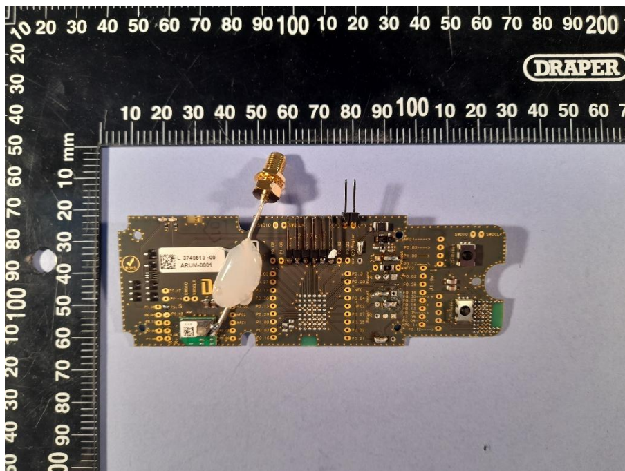
EUT for conducted measurements
