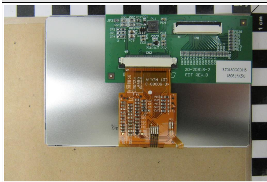
LCD Bottom View
