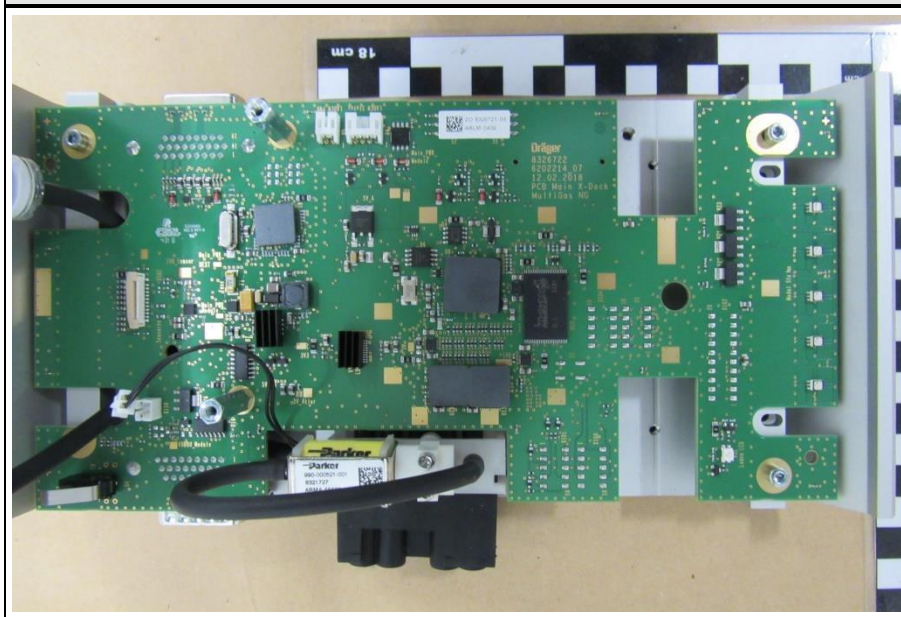
Main PCB Top
