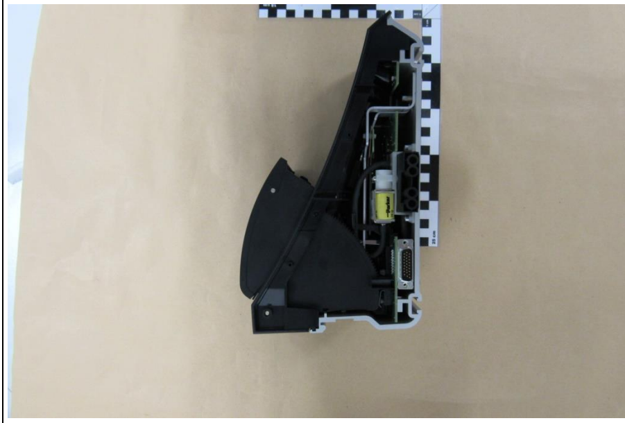
L-Side View
