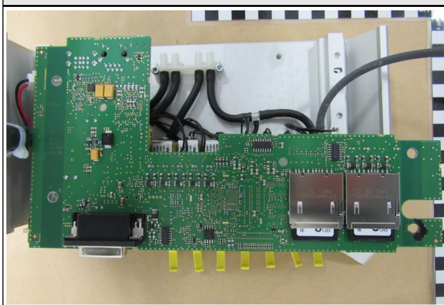
Main PCB Bottom
