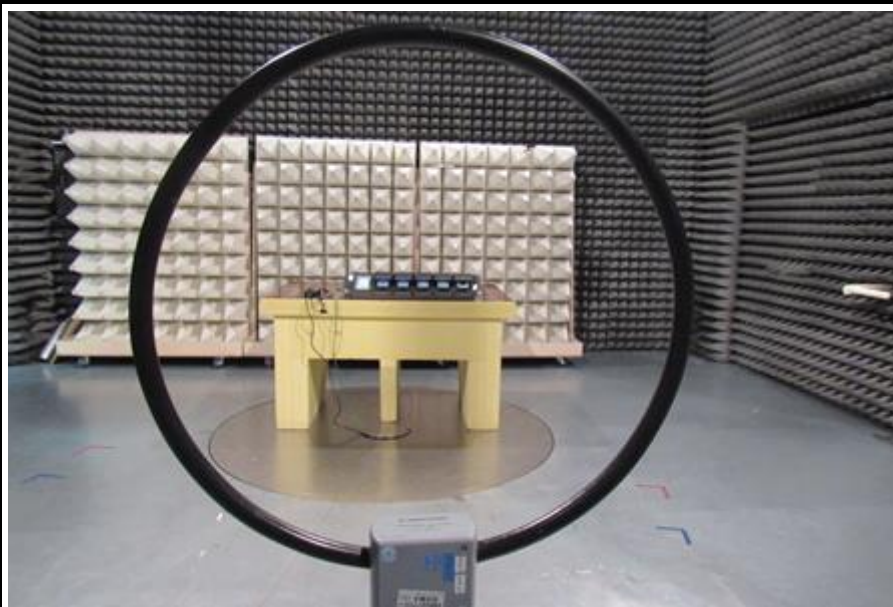
TEST SETUP 1 EUT CONFIGURATION 2 RADIATED EMISSION
