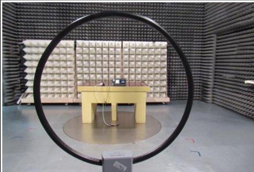
TEST SETUP1 EUT CONFIGURATION 1 RADIATED EMISSION
