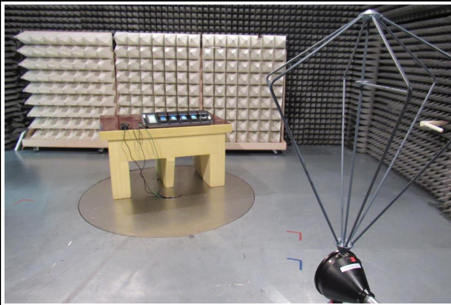
TEST SETUP 1 EUT CONFIGURATION 2 RE 30-200 MHz
