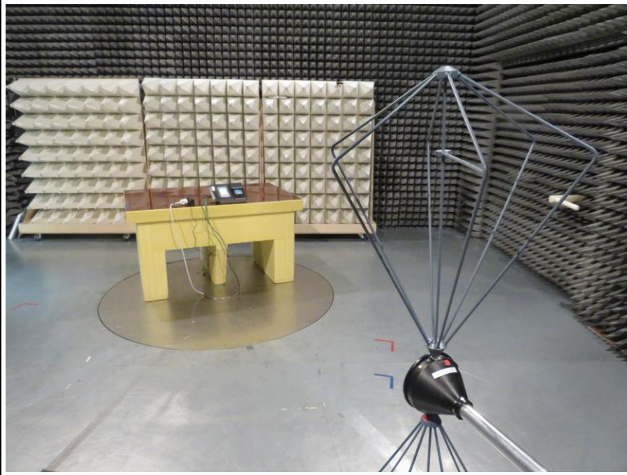
TEST SETUP 1 EUT CONFIGURATION 1 RE 30-200 MHz
