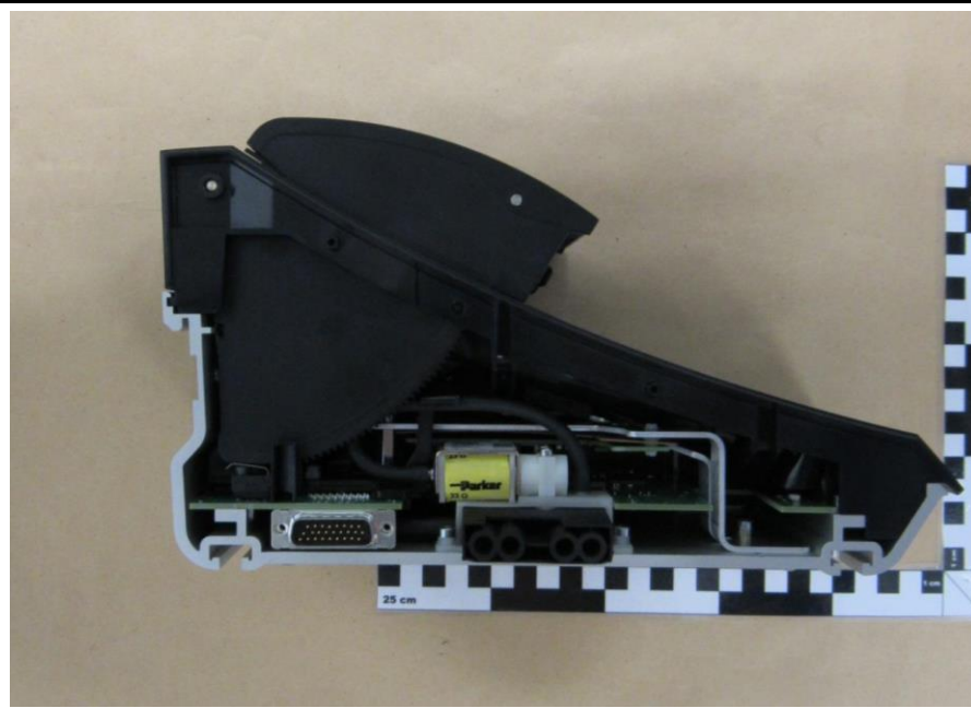
L-Side View
