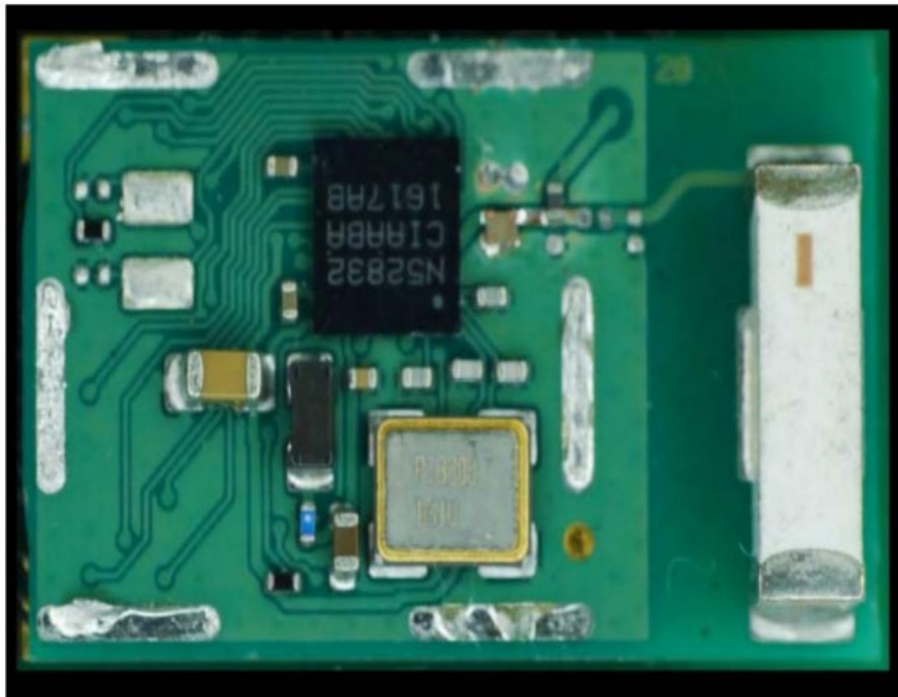
EUT 1 PCB bottom view modul open
