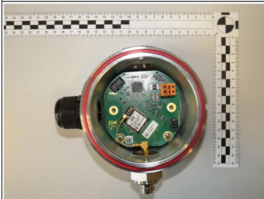
EUT 2 PCB inside Device
