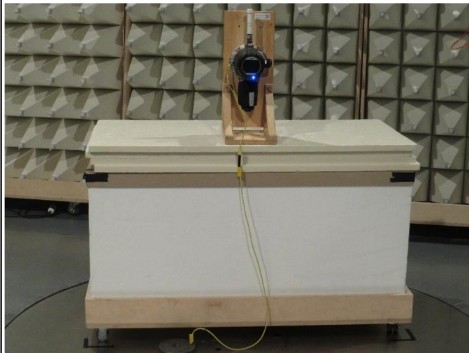
EUT 1 battery setup
