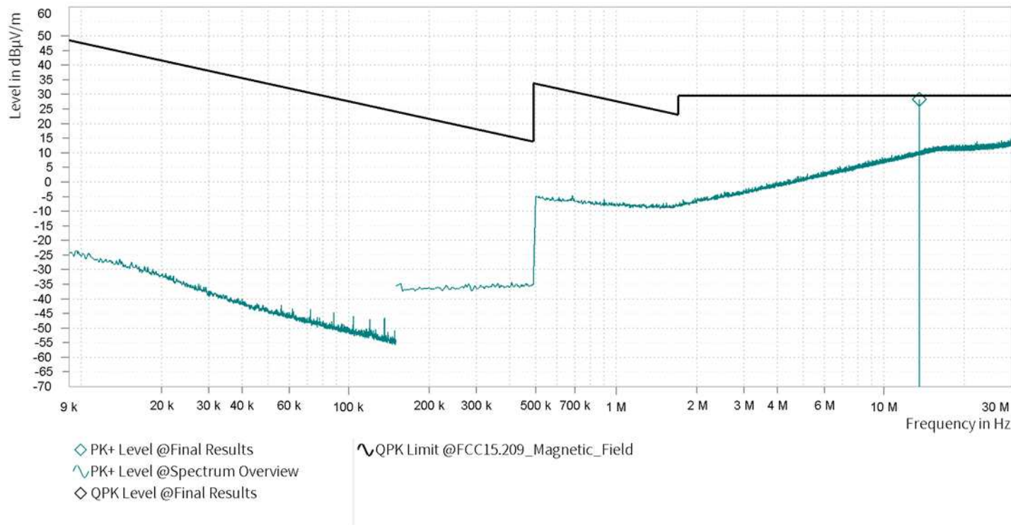
Plot no. 2: Radiated emissions 9 kHz – 30 MHz, EUT lying (see photos in annex B for EUT position)
