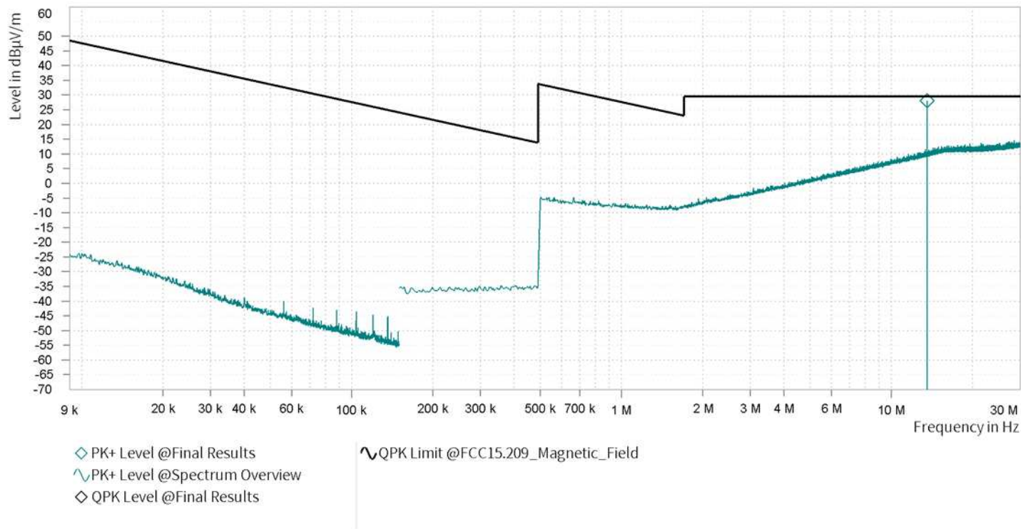
Plot no. 3: Radiated emissions 9 kHz – 30 MHz, EUT standing (see photos in annex B for EUT position)
