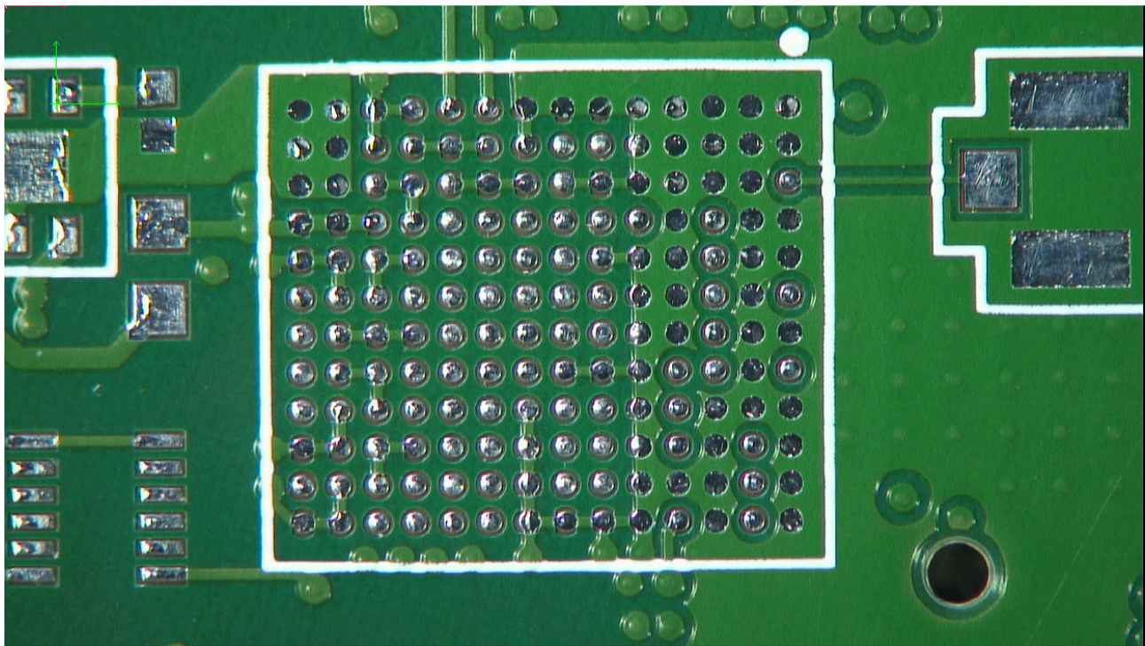
PHOTO OF PCB POSITION OF THE WI-FI RADIO MODULE
