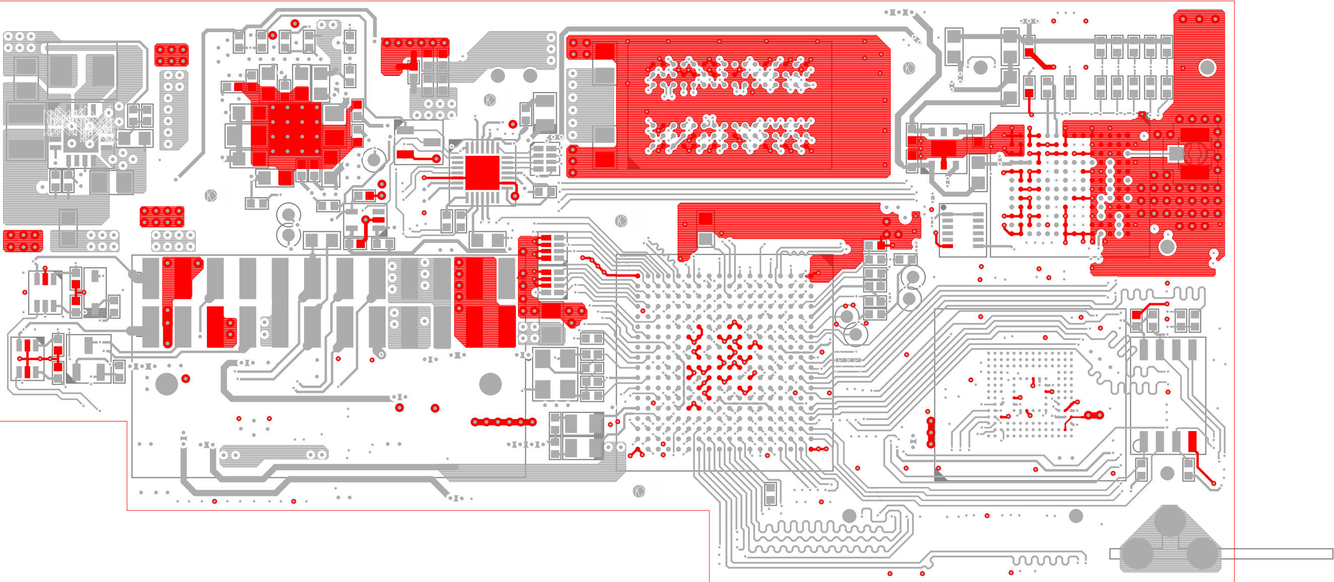
Component Side (L1)
