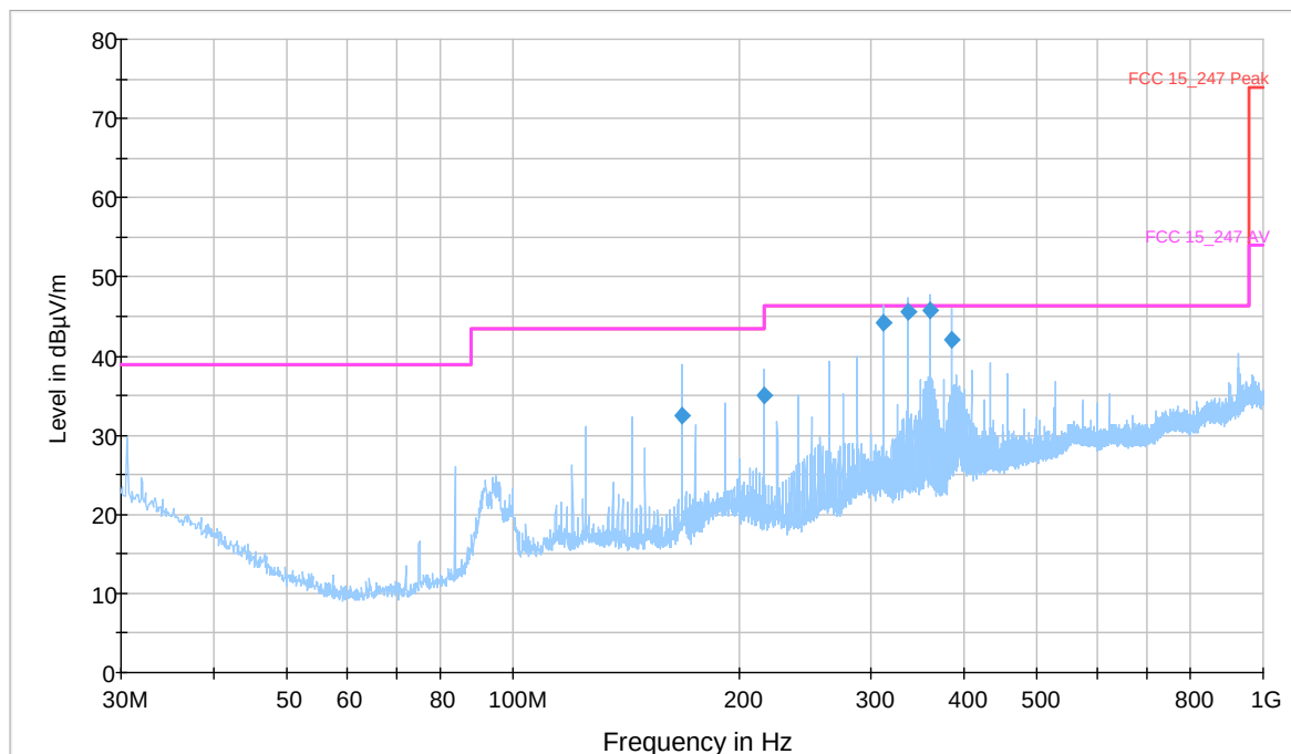
FCC_15_247_RADIATED_SPURIOUS_VERTICAL
