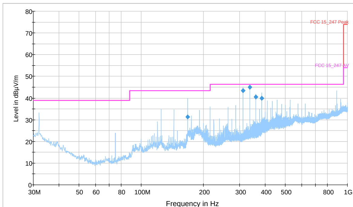
FCC_15_247_RADIATED_SPURIOUS_VERTICAL
