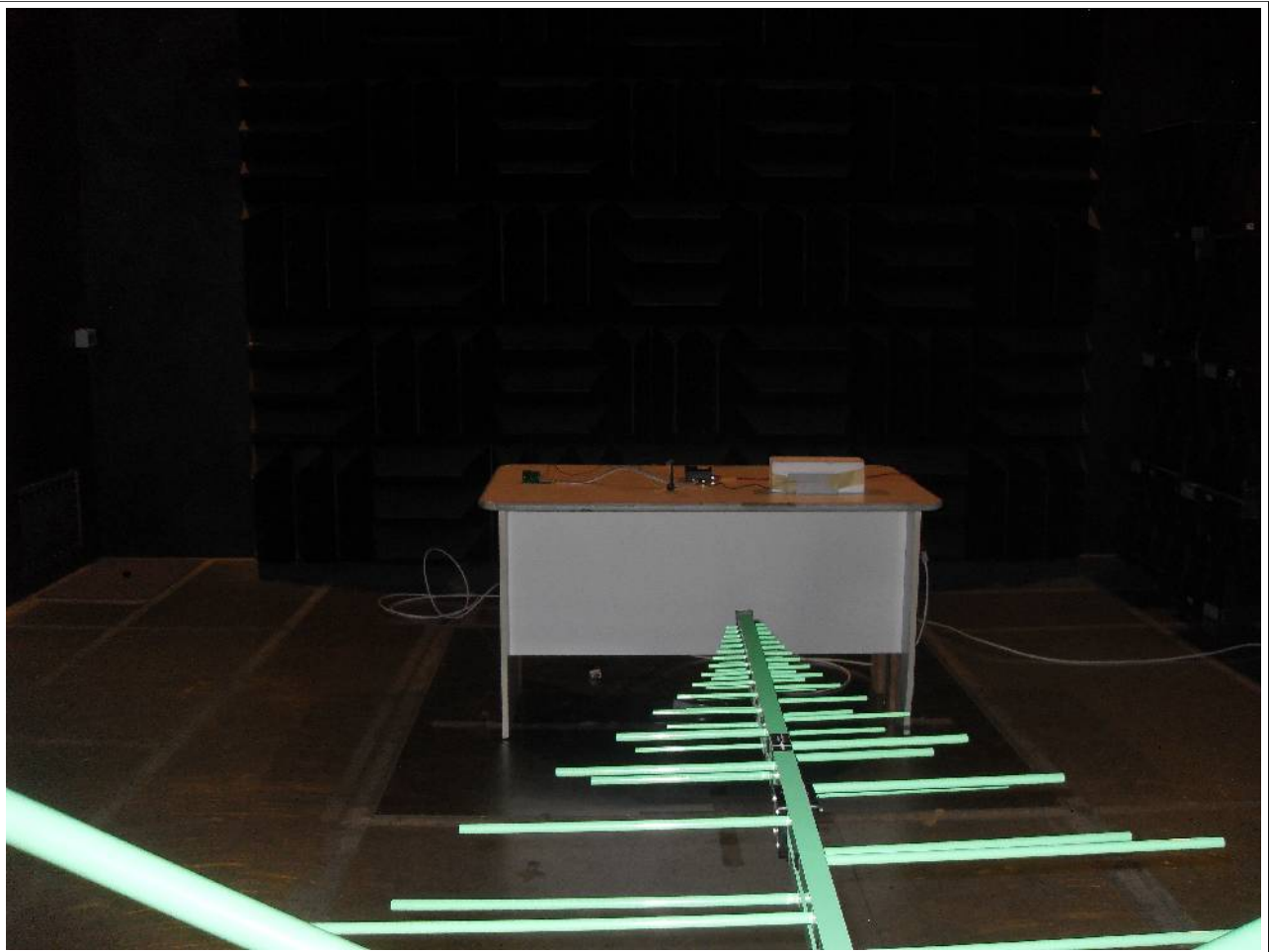
Radiated Emissions
