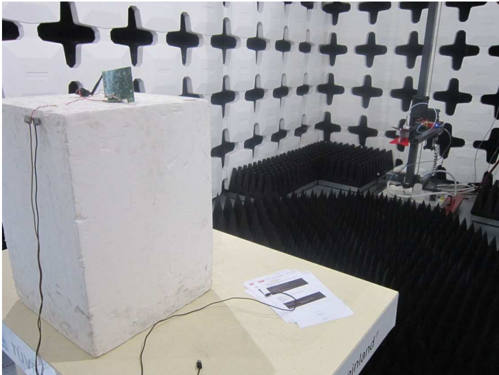
PHOTOS TEST SET_UP
