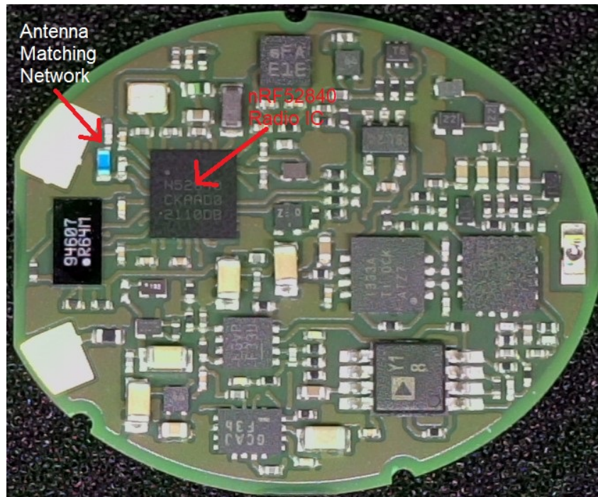
Figure 1: PCBA Top View
