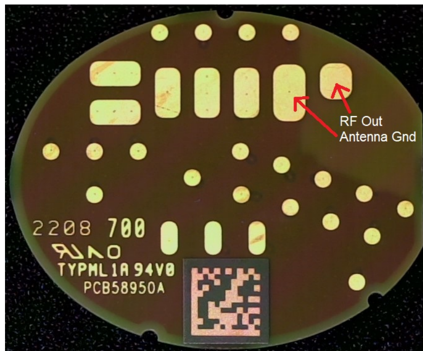
Figure 2: PCBA Bottom View
