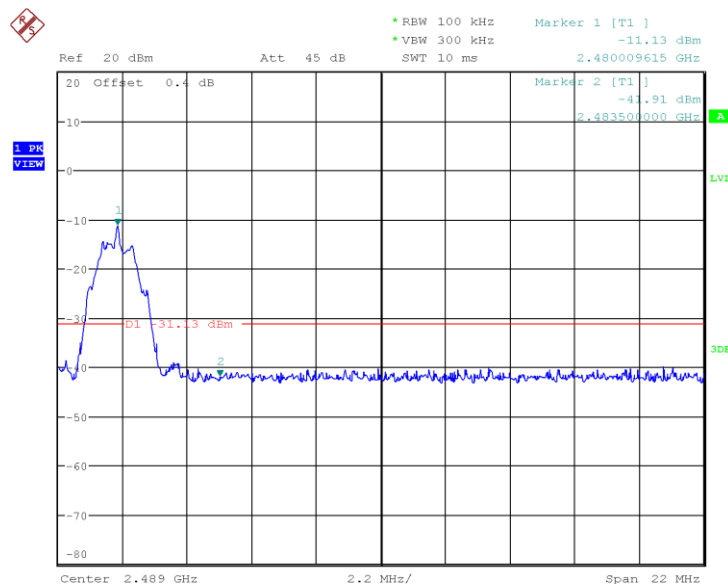
Figure 28: 2480MHz, 2Mbps Upper Band Edge
