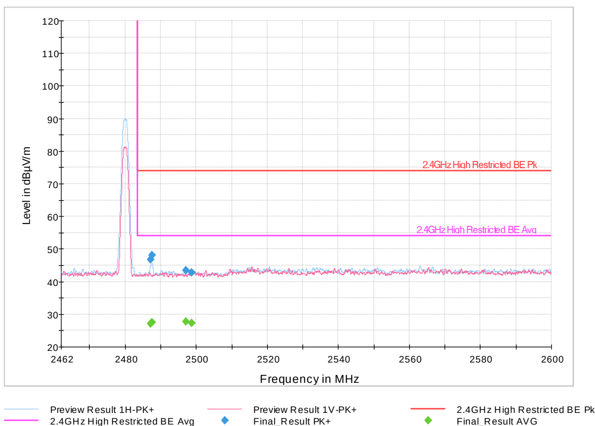
Figure 38: Restricted Band Edge, High, 2480MHz, 1 Mbps
