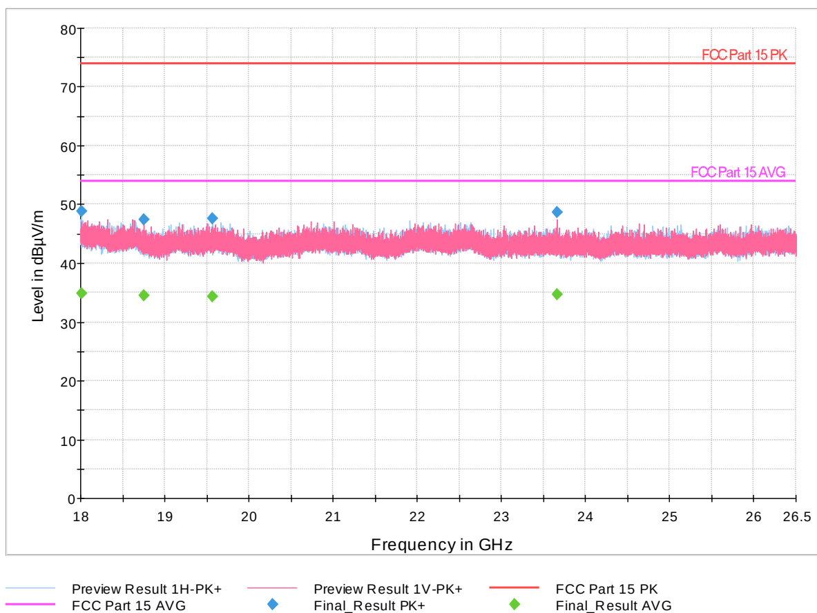
Figure 46: Radiated Spurious Emissions 18GHz – 26.5GHz, 2480MHz, 1Mbps
