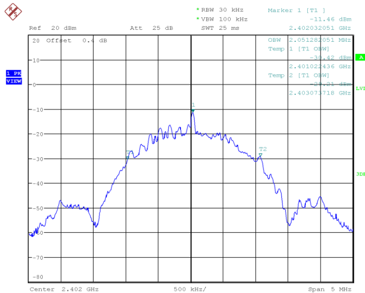
Figure 16: 2402MHz, 2Mbps, 99% Bandwidth
