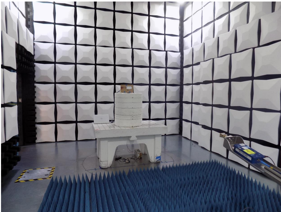
Figure 5: Test Setup for Radiated Emissions 18-26.5GHz - Front View
