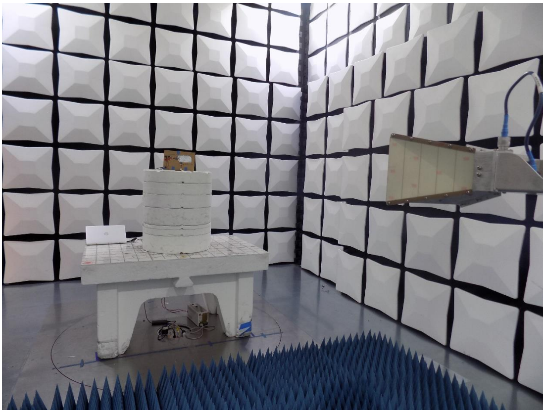
Figure 3: Test Setup for Radiated Emissions 1-18GHz - Front View
