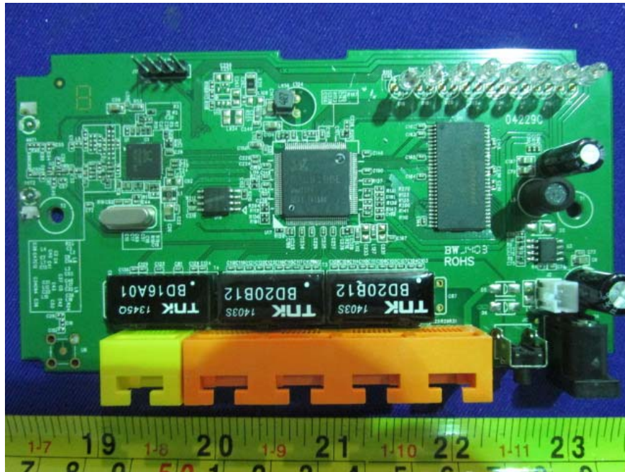
EUT – Main Board Top without Heat-Sink View
