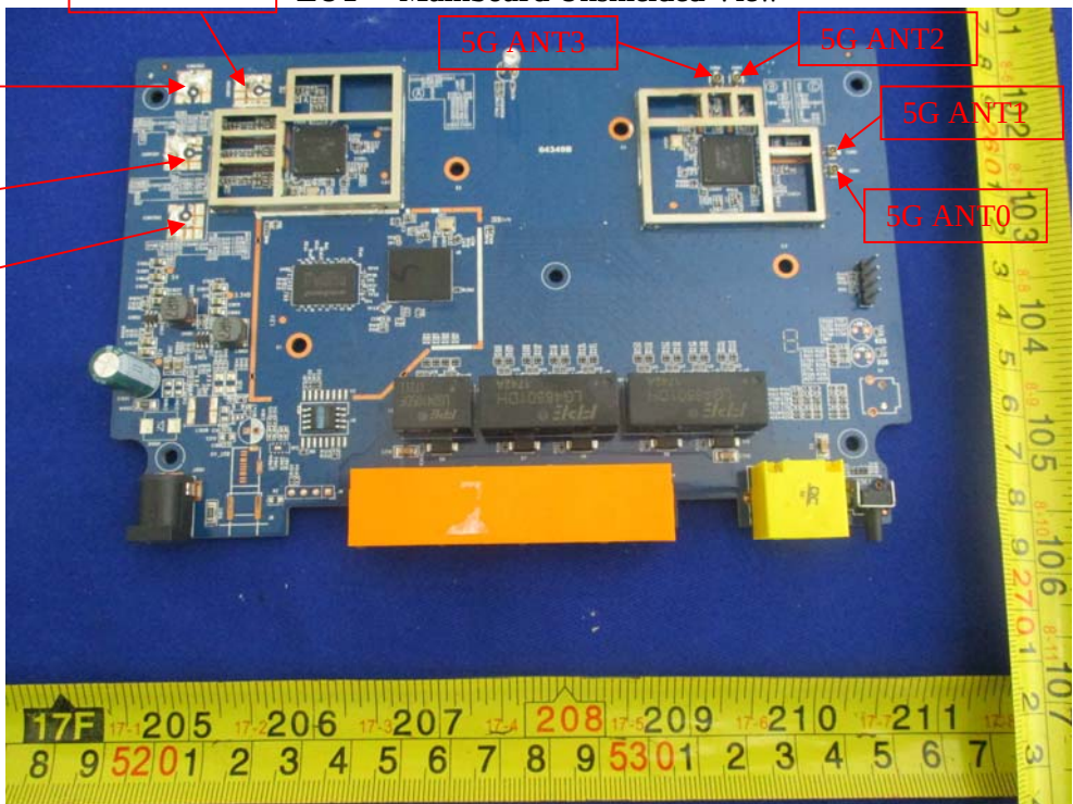
EUT – Mainboard Unshielded View
