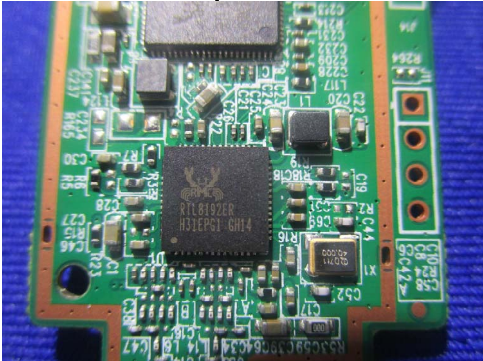
EUT – Chip RTL8192ER View
