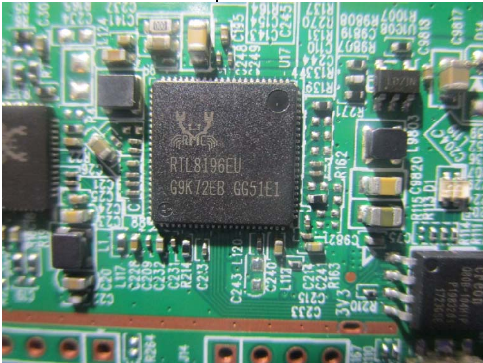
EUT – Chip RTL8196EU View
