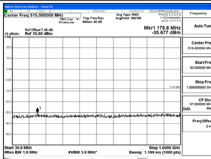
GPRS1900_661_30~1000_-35.68_-13_PASS
