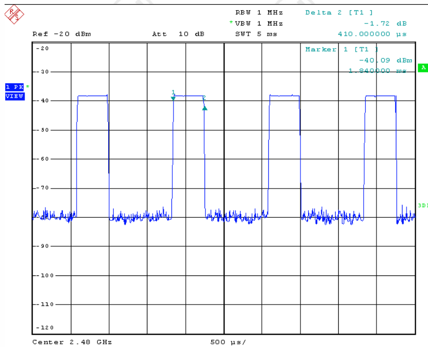
2480 MHz_DH1
