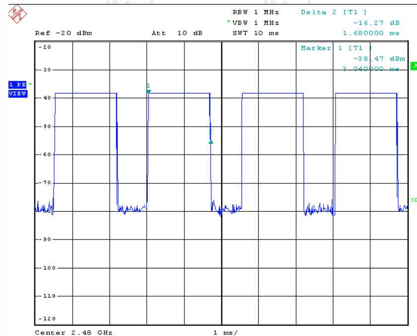
2480 MHz_DH3
