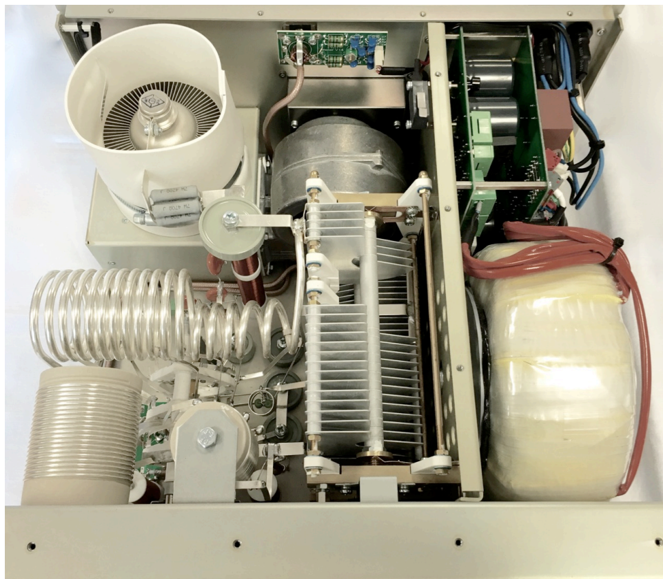
Fig. 3 Top front view
