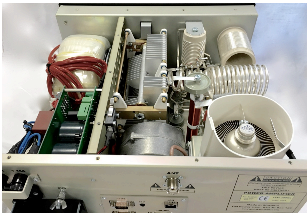
Fig. 4 Top back view
