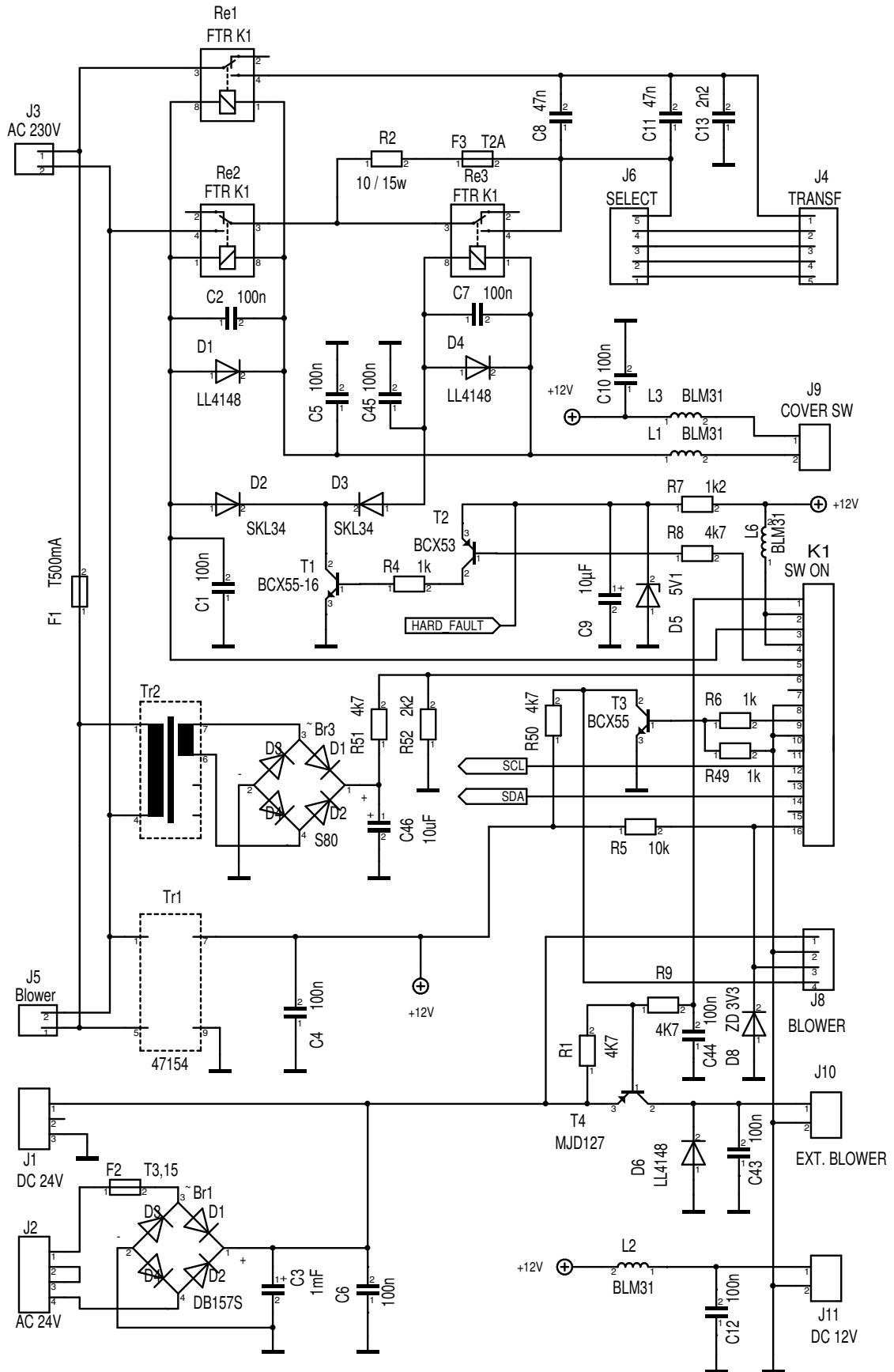
SW ON board OM2000A+ 1/2
