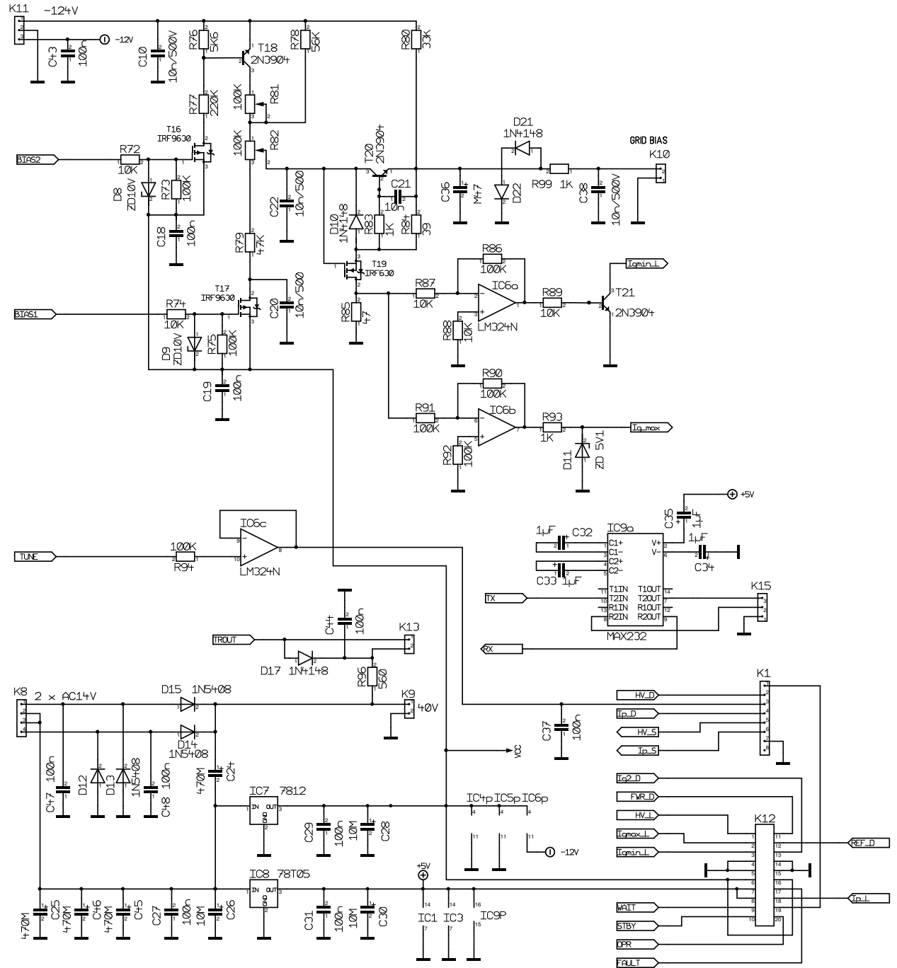
Control board V11
