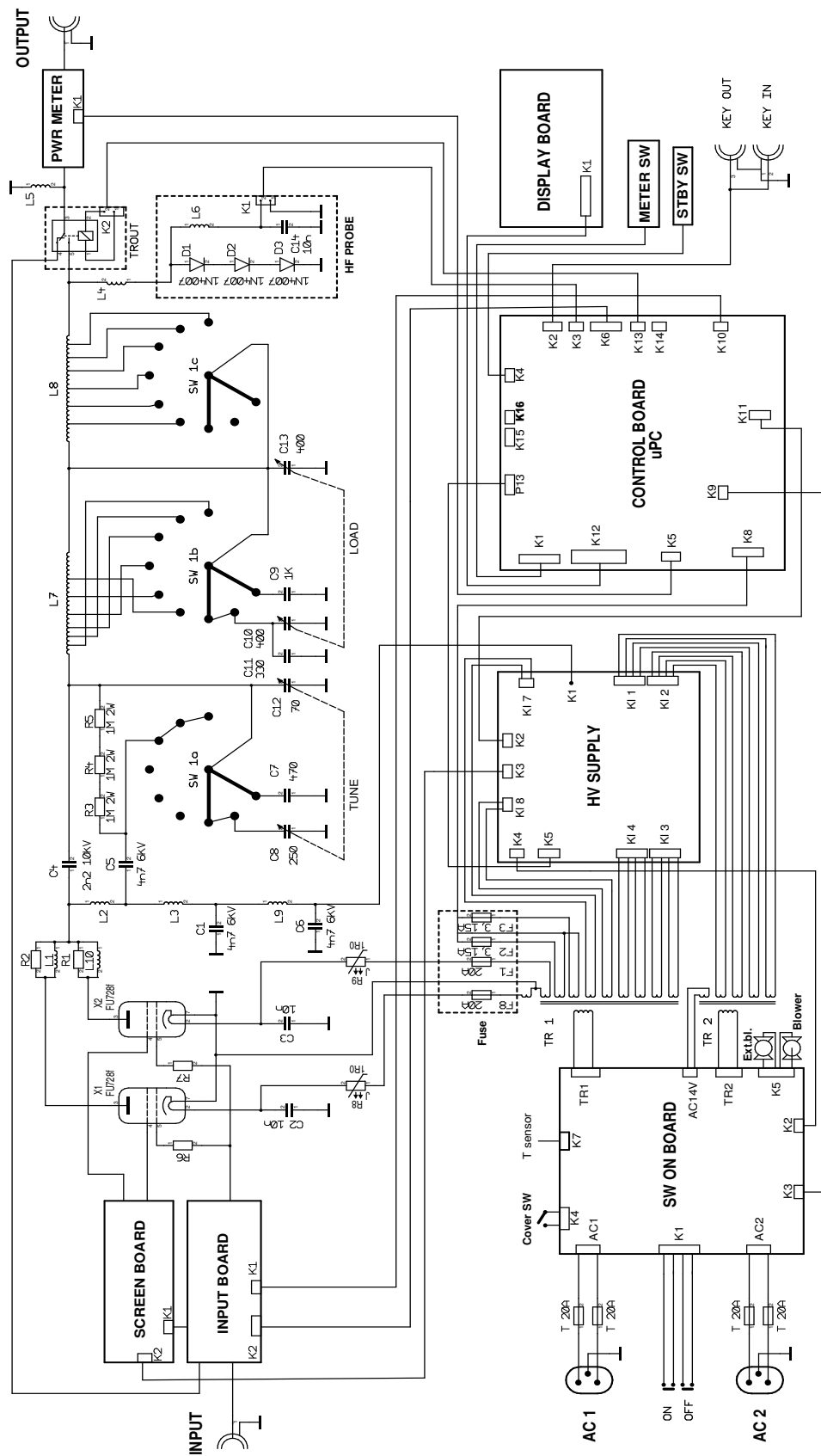
OM 4000HF Block diagram
