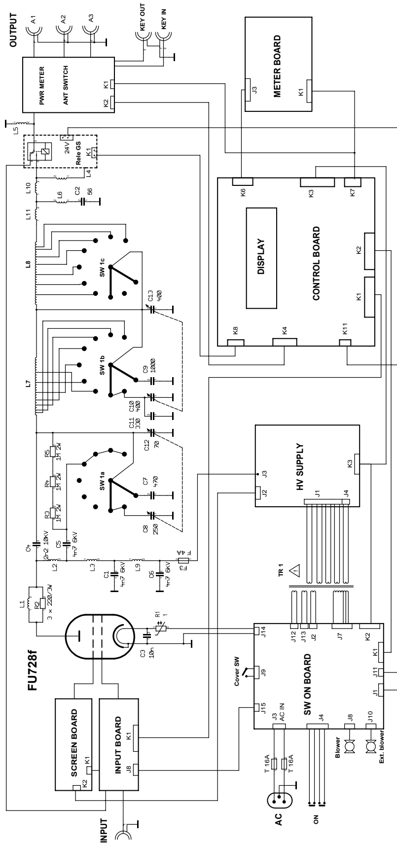
OM 2000+ block diagram
