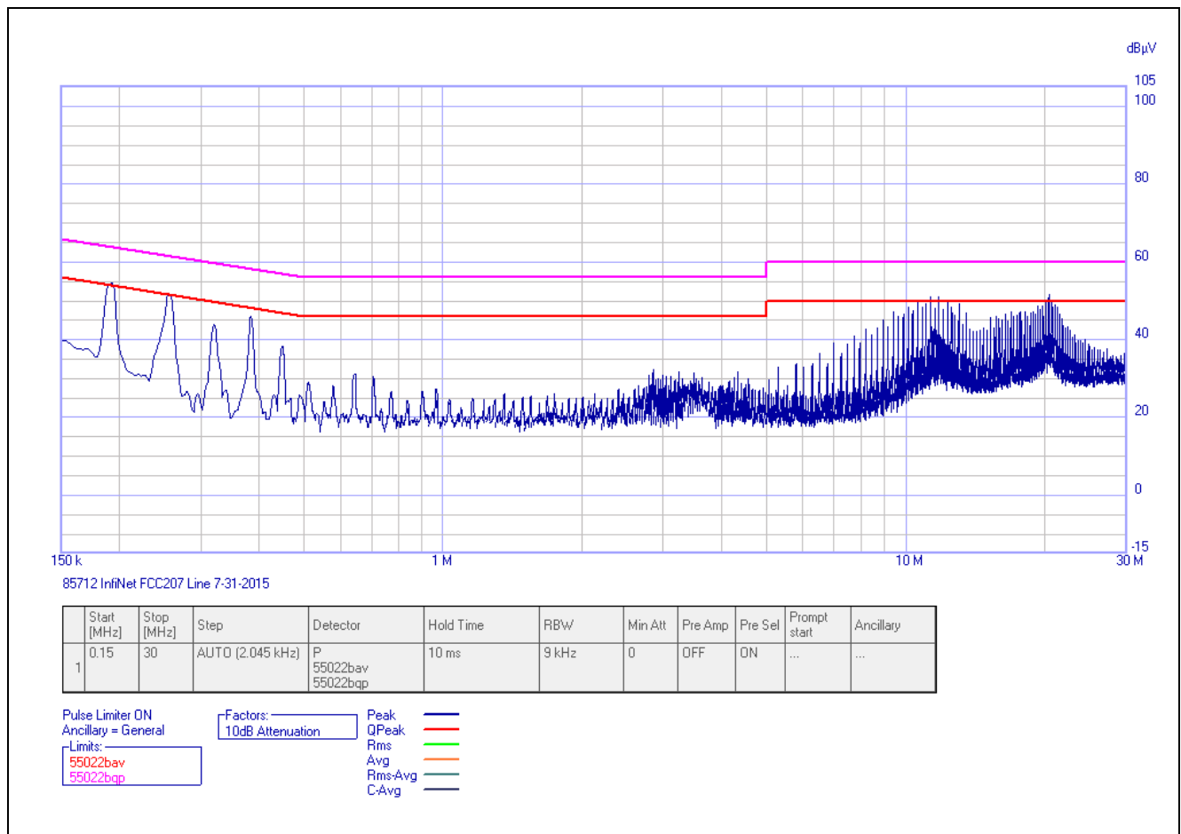
Plot 159. Conducted Emissions, Phase Line
