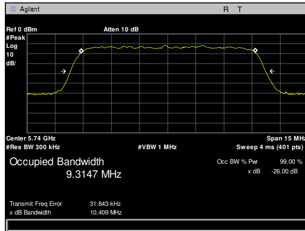
Plot 17. 26 dB Occupied Bandwidth, Low Channel, 10 MHz, Port 1
