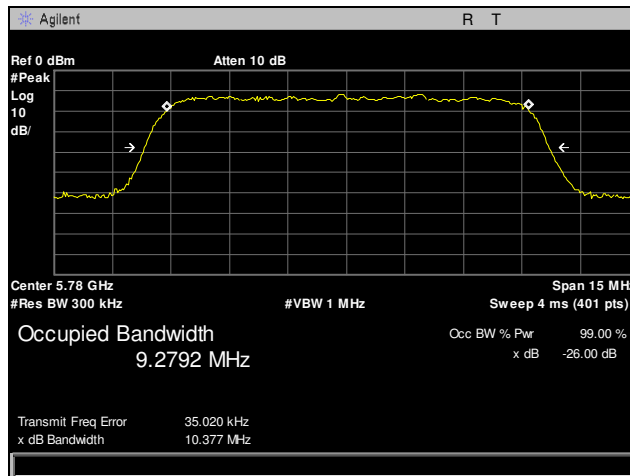
Plot 18. 26 dB Occupied Bandwidth, Mid Channel, 10 MHz, Port 1
