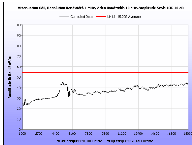
Plot 109. Radiated Spurious Emissions, Low Channel, 20 MHz, 1 GHz – 18 GHz, 23 dBi Antenna, Average
