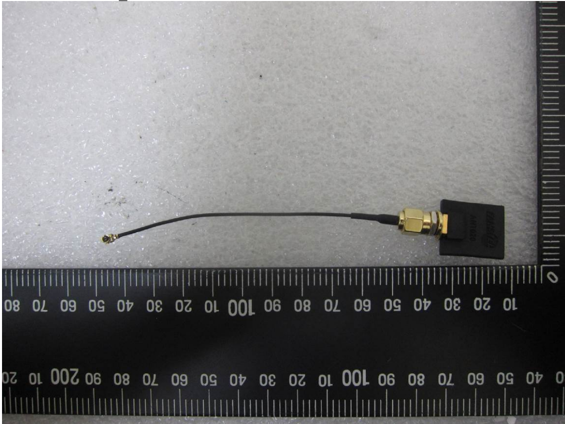
EUT-13. BC40P_ANT
