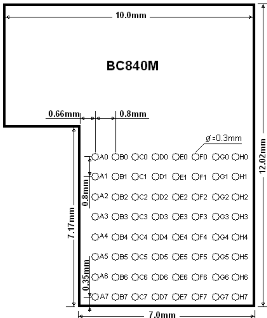
BC840M mechanical drawings, top view.
