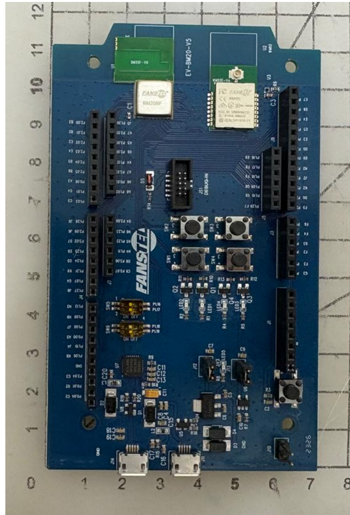
Figure 1 2.4G Antenna
