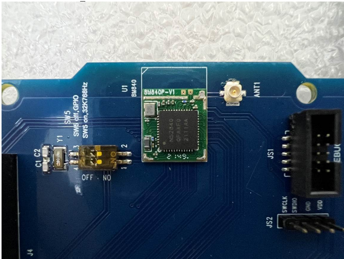
EUT-3. BM840P_Module
