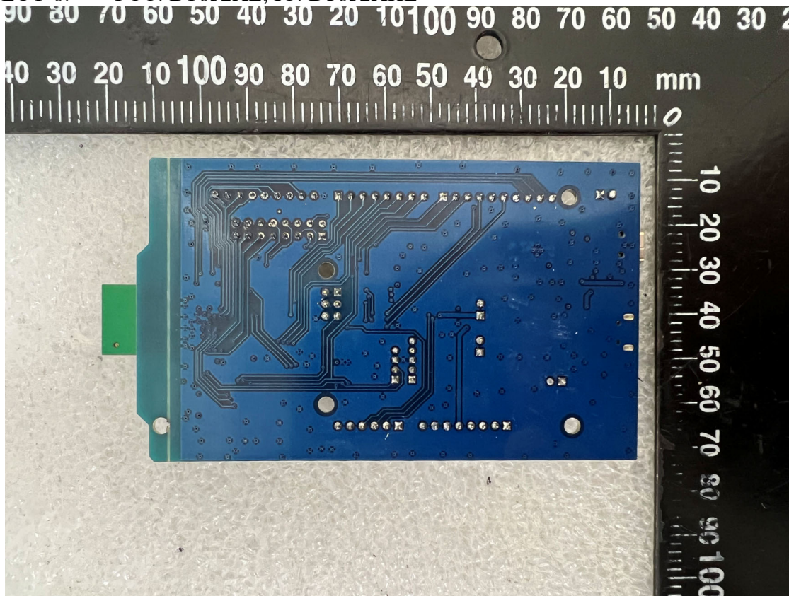
EUT-8. FCC: BT832XE, IC: BT832XHE
