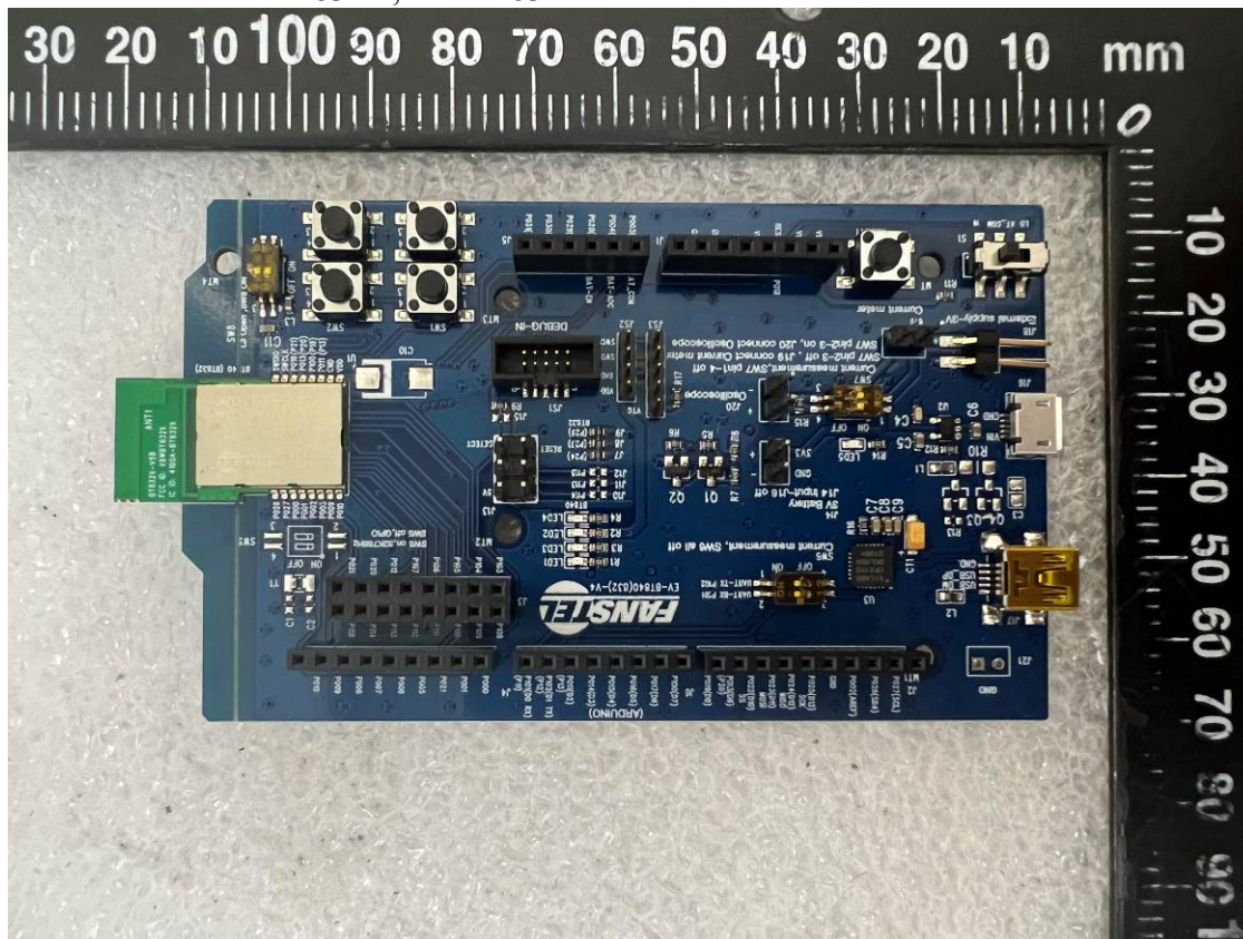
EUT-1. FCC: BT832X, IC: BT832XH
