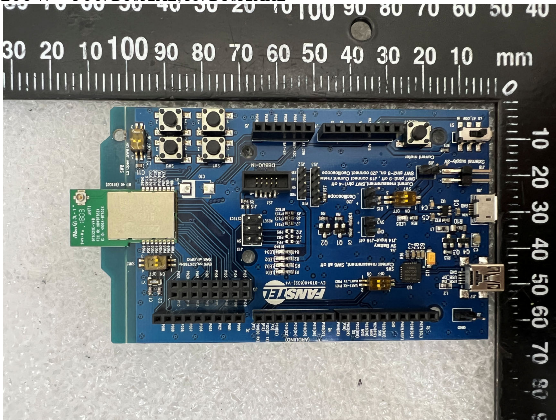
EUT-7. FCC: BT832XE, IC: BT832XHE
