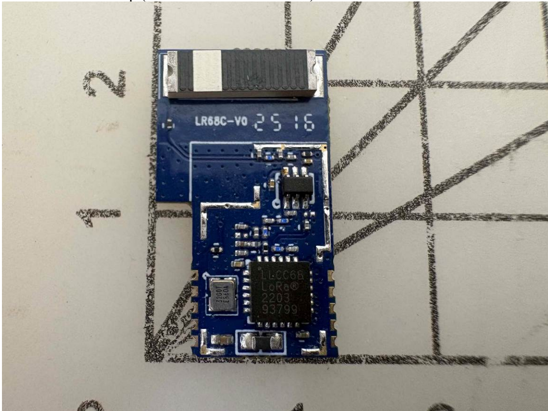
EUT-20. ANT Chip (WAN031003F0391SM03)
