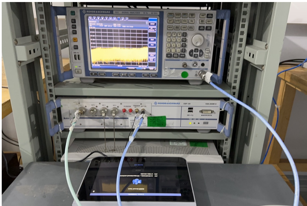
DFS:
