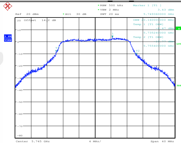
11AC20SISO_Ant1_5745
