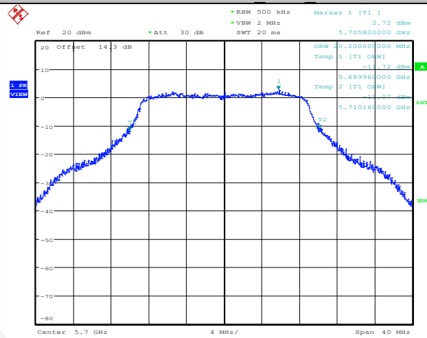
11AC20SISO_Ant1_5700
