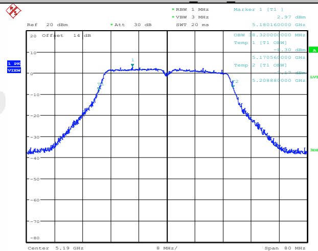
11AC40SISO Ant1 5190
