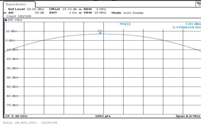
2DH1_Ant1_2480
