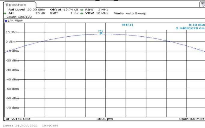
3DH1_Ant1_2441
