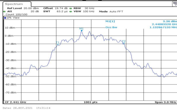
2DH1_Ant1_2441
