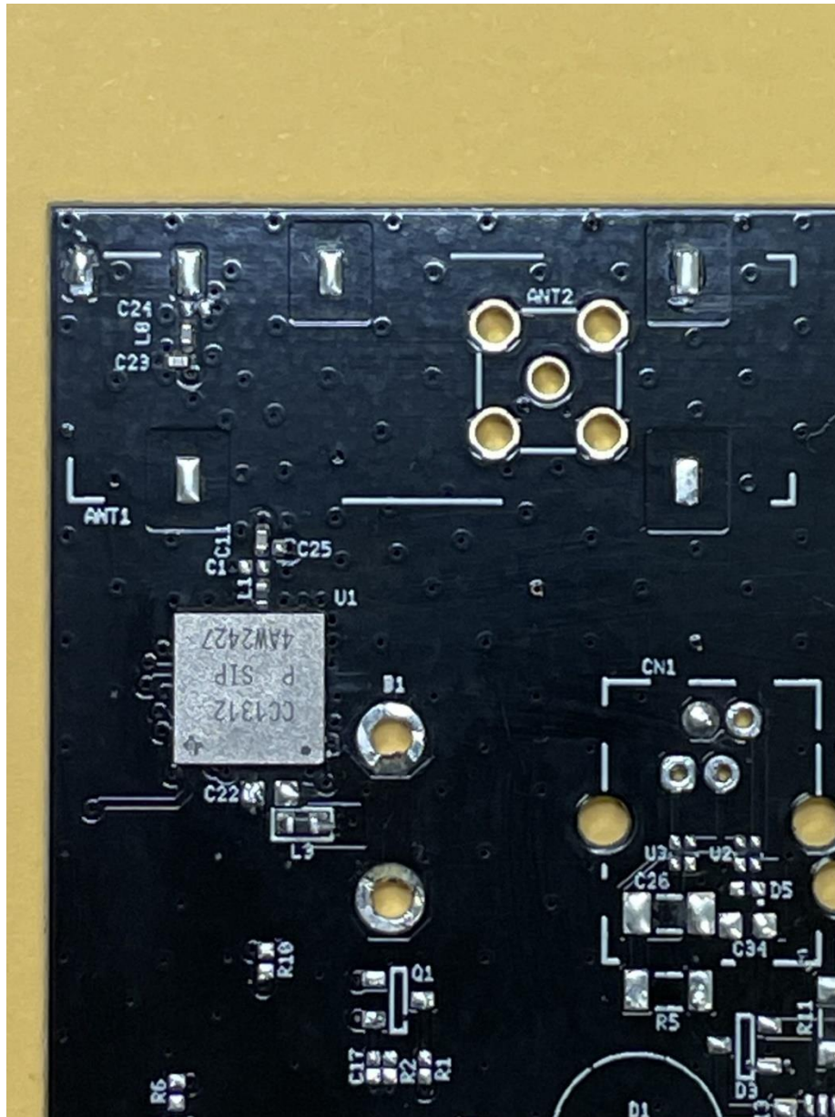
13. PCB under antenna
