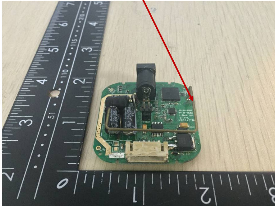
Z-WAVE Antenna
