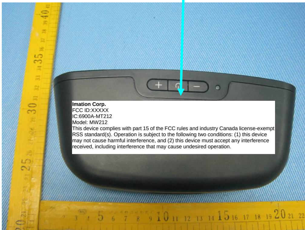
Proposed Label Location on EUT EUT Back View/ proposed IC Label Location
