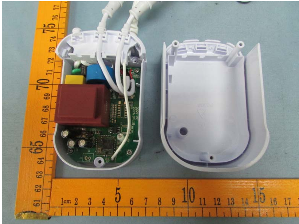
ZW095-A - Internal View
