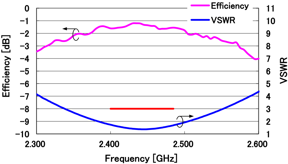
Efficiency and VSWR
