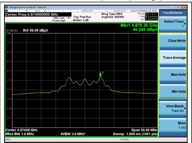
Middle channel 2 nd Spurious (Average)
