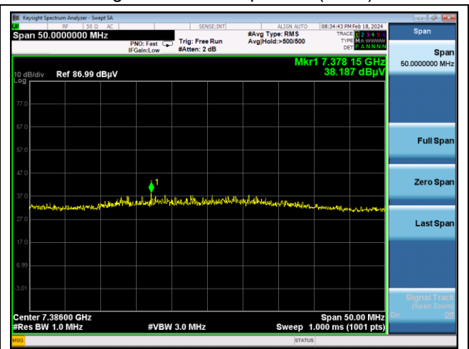
High channel 3 rd Spurious (Peak)
