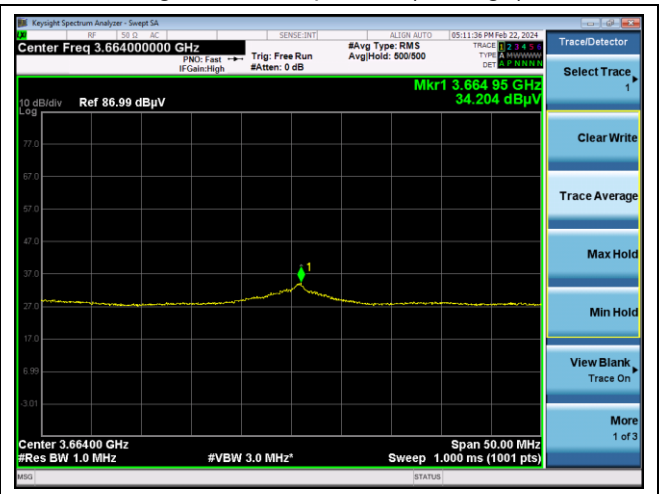
High channel Spurious (Average)
