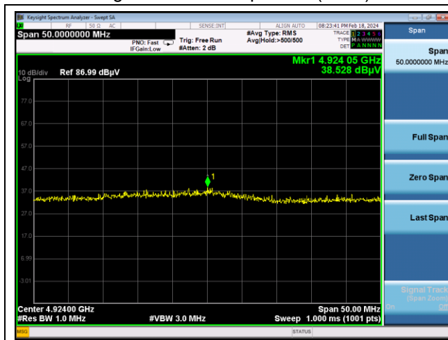
High channel 2 nd Spurious (Peak)
