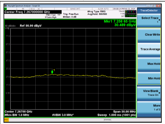
Low channel 3 rd Spurious (Average)
