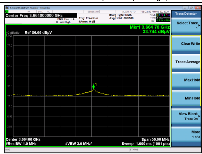
Middle channel Spurious (Average)
