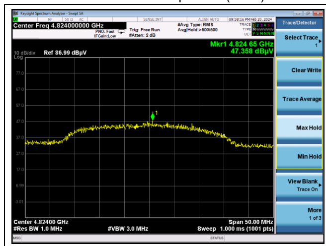
Low channel 2 nd Spurious (Peak)
