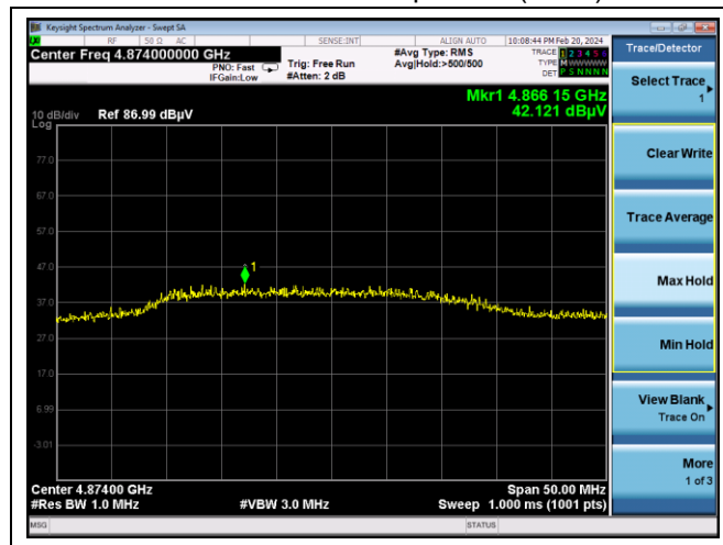
Middle channel 2 nd Spurious (Peak)
