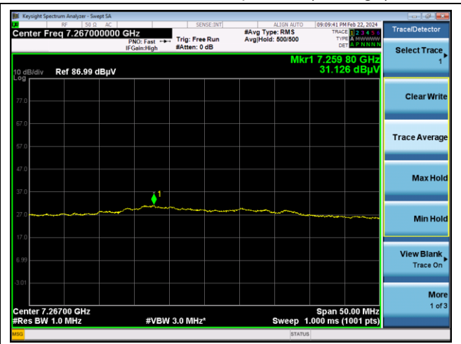
Middle channel 3 rd Spurious (Average)
