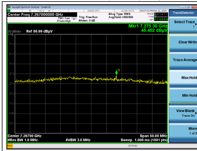
Low channel 3 rd Spurious (Peak)
