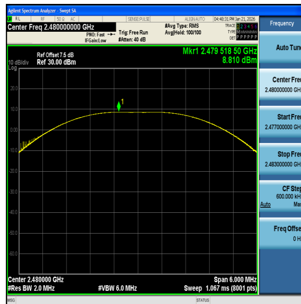
BLE_2M-Ant1-2480-PASS
