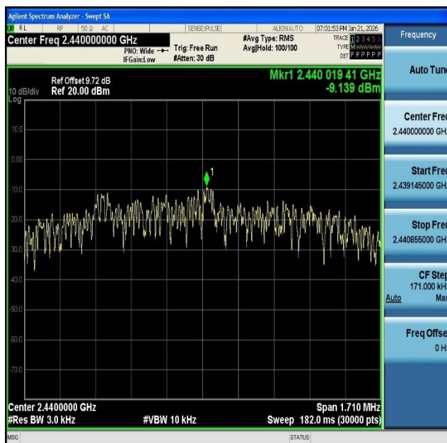
BLE_2M-Ant1-2440-PASS
