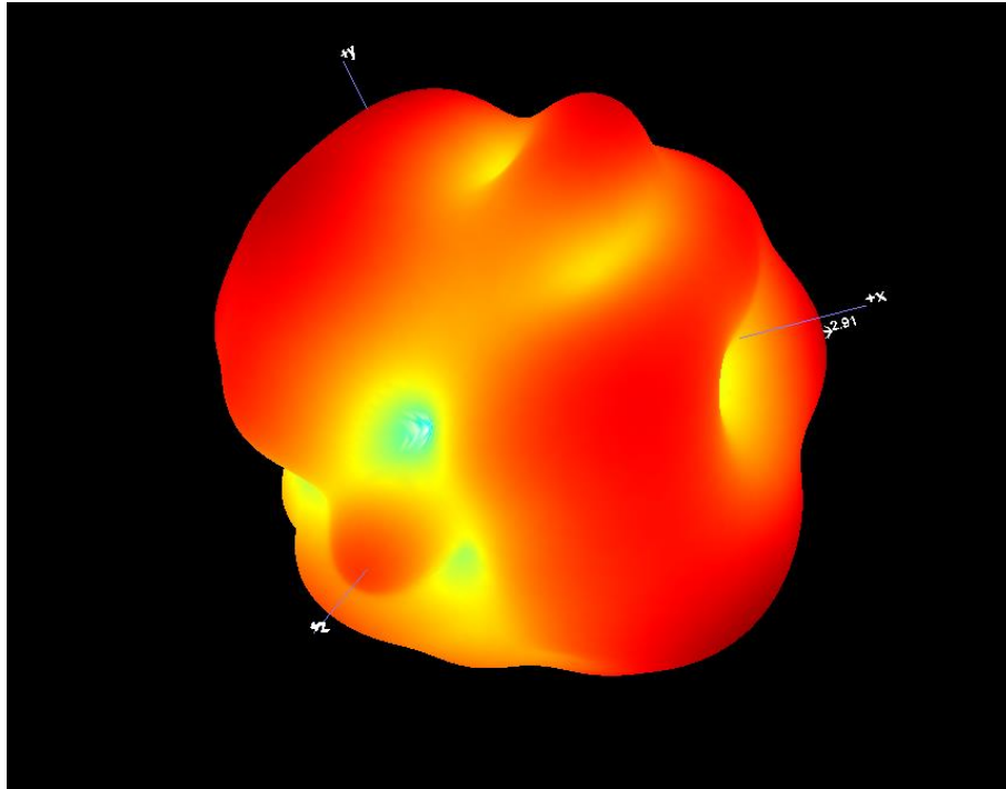
B1.1 3D Pattern for 2402MHz
