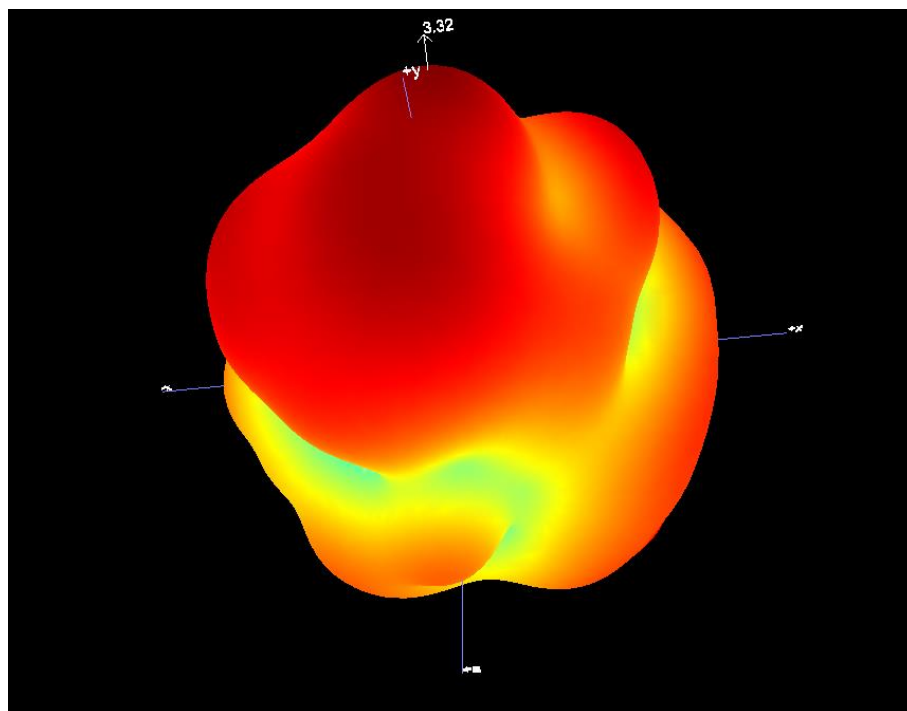
B1.3 3D Pattern for 2480MHz
